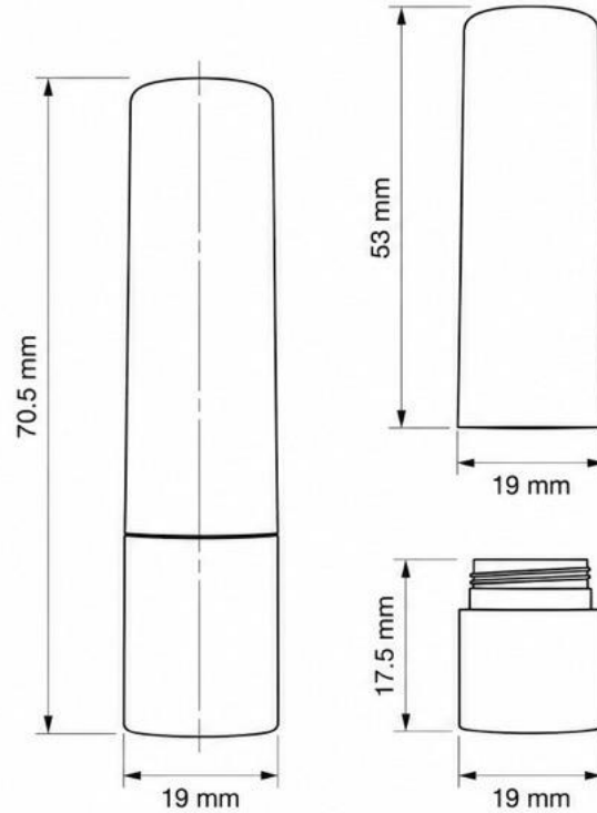
TEKNİK ÇİZİM / TECHNICAL DRAWING
